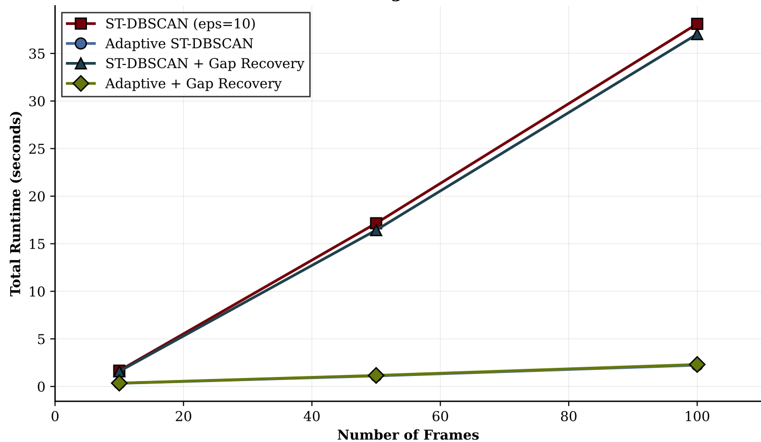
Runtime Scaling with Dataset Size
